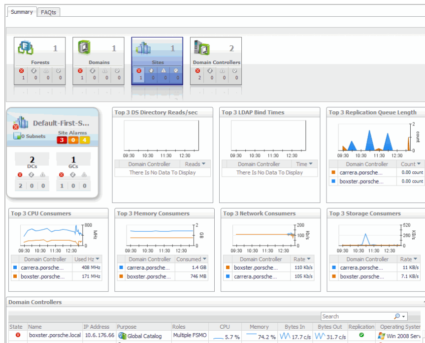
Figure 30. Site Explorer Summary view
