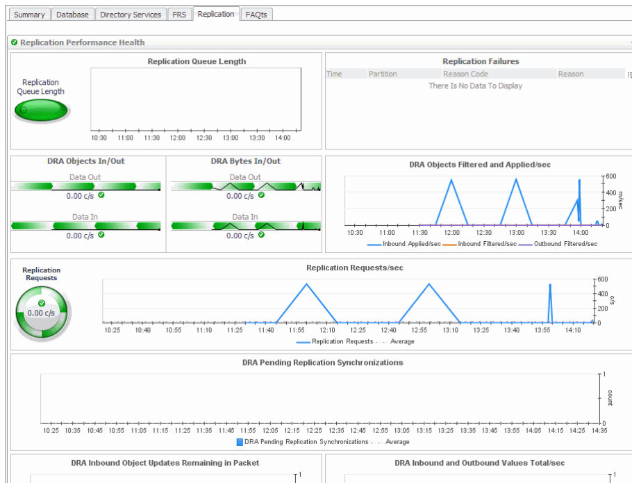
Figure 40. Domain Controller Replication view
